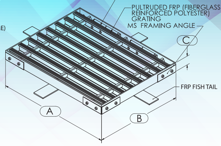
FRP Grating C/W FRP Frame
