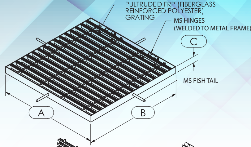
FRP Grating C/W MS Frame
