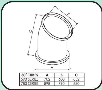
30 Deg Tube
