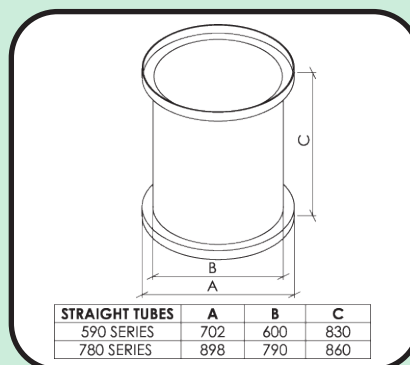
Straight Tube
