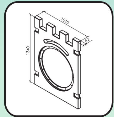
• Bracket Panel-780
