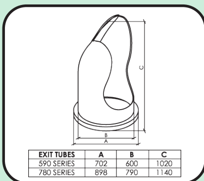
Exit Tube
