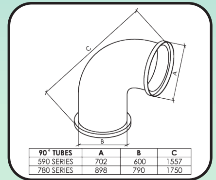
90 Deg Tube
