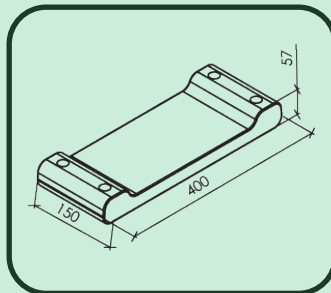
• Swing Seat
