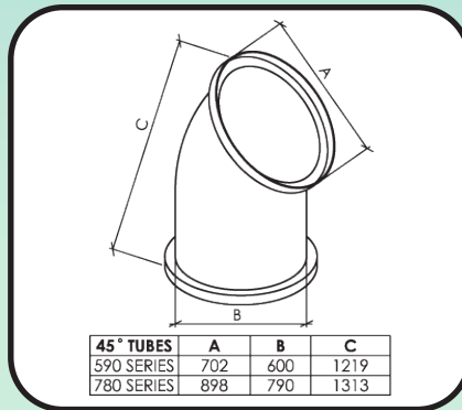
45 Deg Tube
