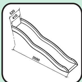
• Short Slide
